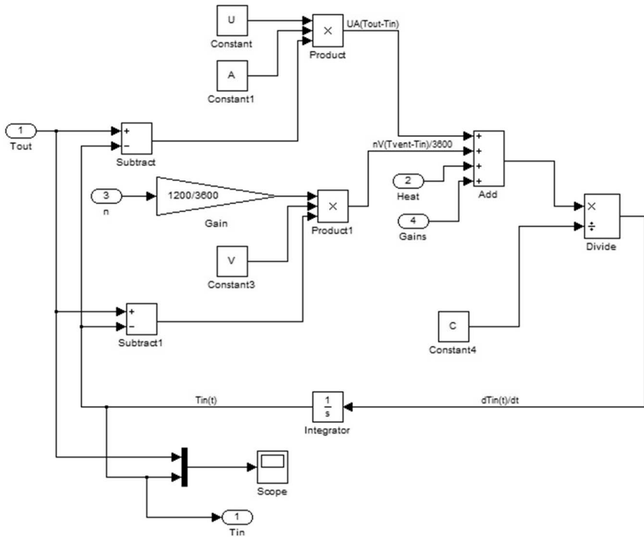
Fig. 2: Building space model
