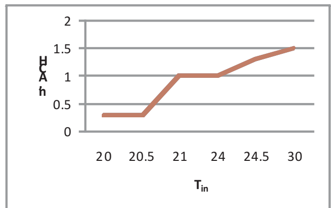
Fig. 3: Number of air changes per hour
