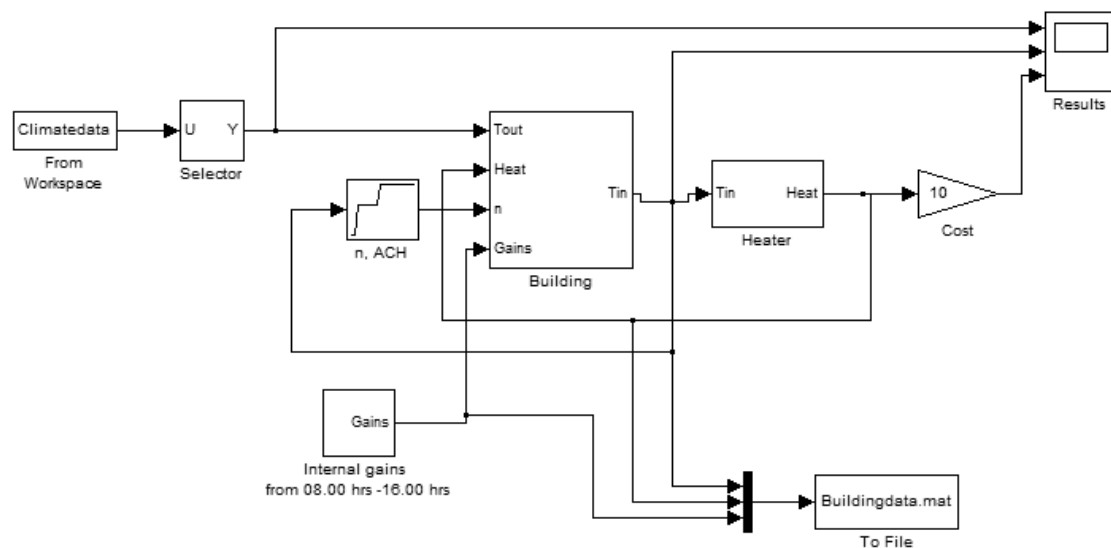
Fig. 1: Overall Building model in Simulink
